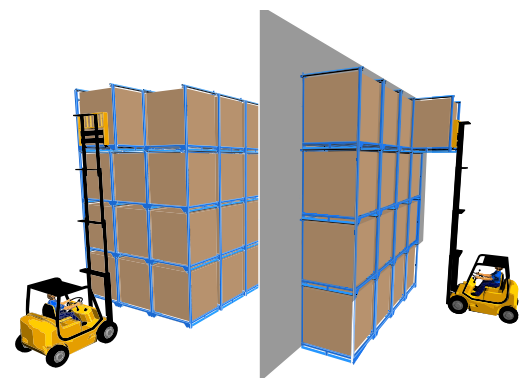
StakRack can be stacked up to 4 high on a level floor and should be positioned against a back wall or back to back
