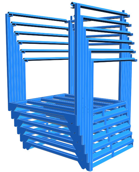
StakRack can be nested for efficient storage.
