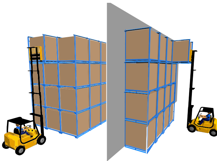
StakRack can be stacked up to 4 high on a level floor and should be positioned against a back wall or back to back
