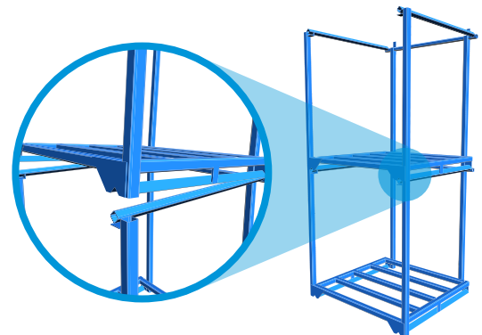
StakRack locate together safely and easily.
